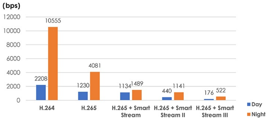
Bandwidth measurement using different Smart Stream generation
