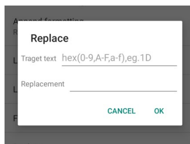
Figure 2-29 Edit Replace
