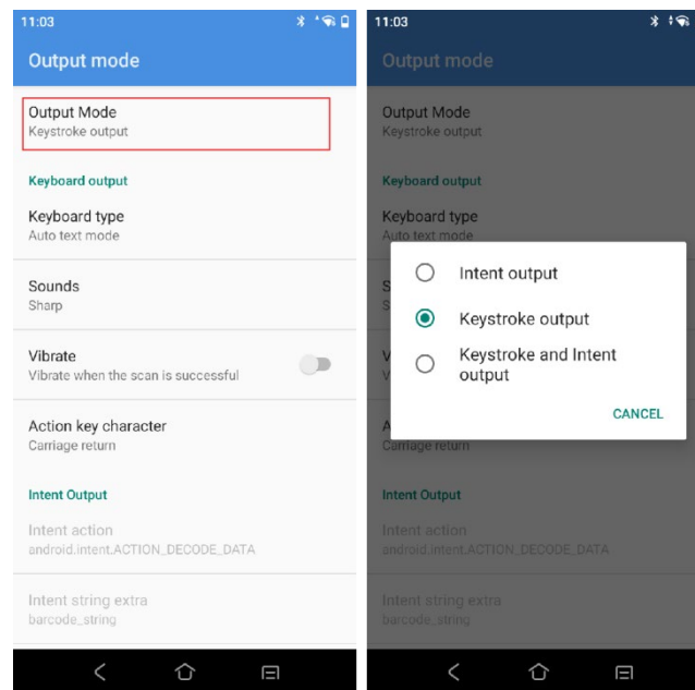
Figure 2-20 keystroke output
