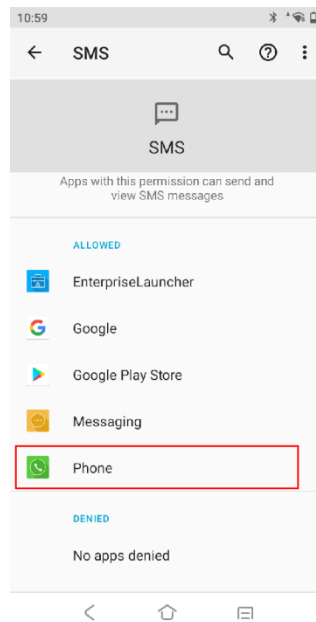
Figure 2-14 SMS Permissions
