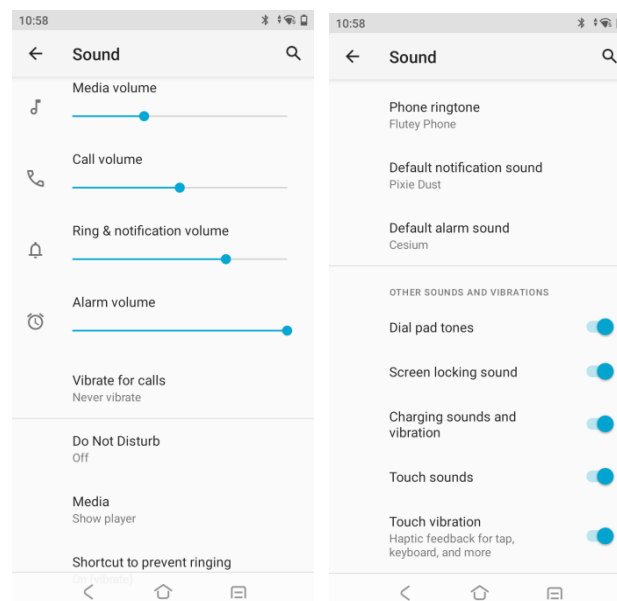
Figure 2-11 Sound Settings
