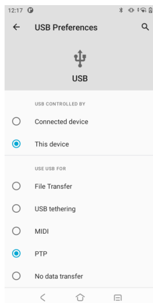
Figure 3-12 PTP
