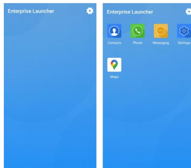
Figure 3-2 user interface
