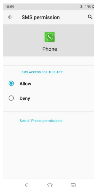
Figure 2-15 SMS permission
