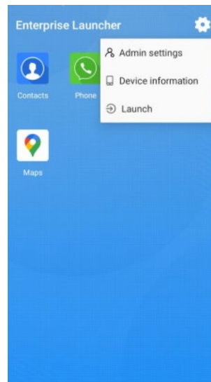
Figure 3-3 menu
