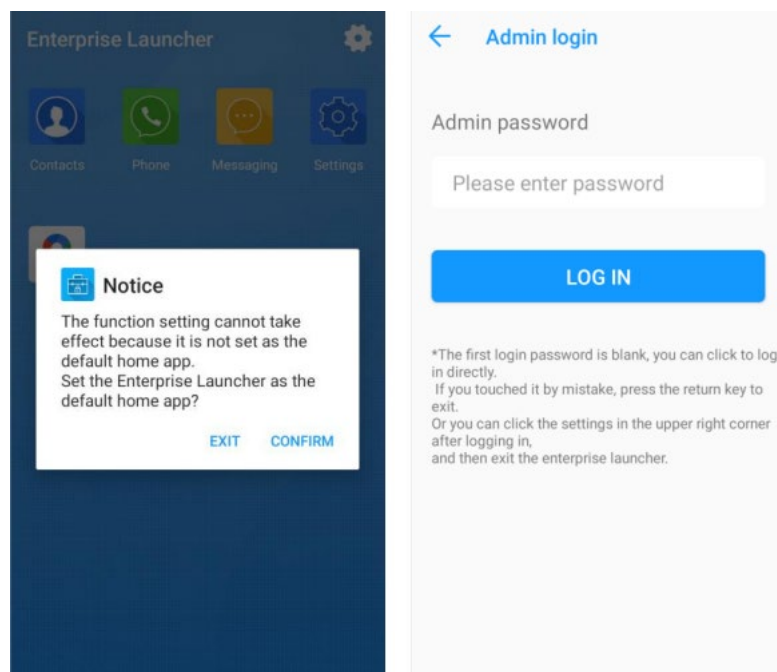
Figure 3-4 Administration login
