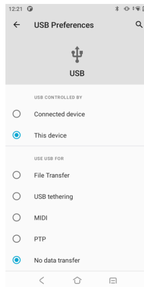
Figure 3-14 Charging mode
