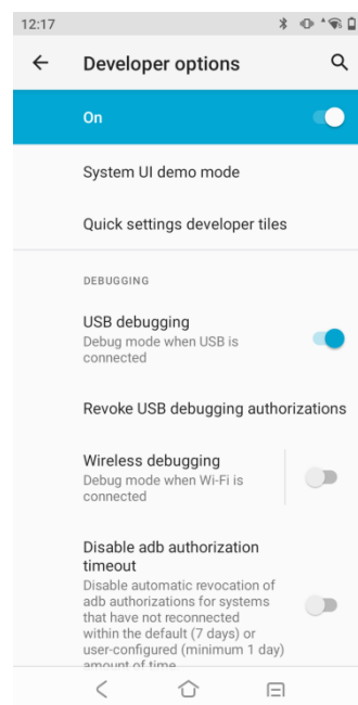
Figure 3-10 USB debugging
