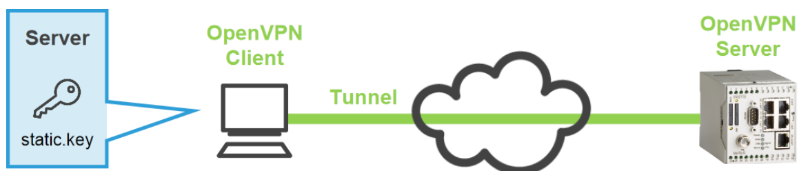
Figure 1: Windows PC as OpenVPN client with authentication via static key
